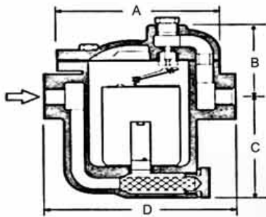
Screwed Ends
