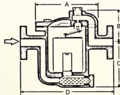
Flange Ends
